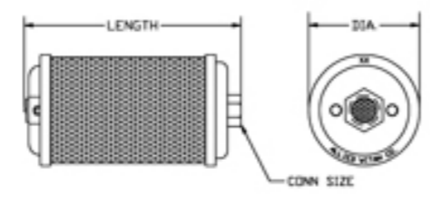
Single Chamber-Female 1/8"-2"
