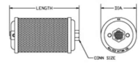
Single Chamber-Female 1/8"-2"
