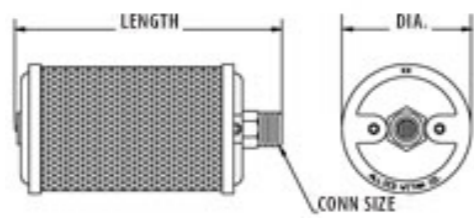
Single Chamber-Male 1/8"-2"
