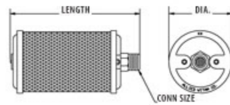
Single Chamber-Male 1/8"-2"
